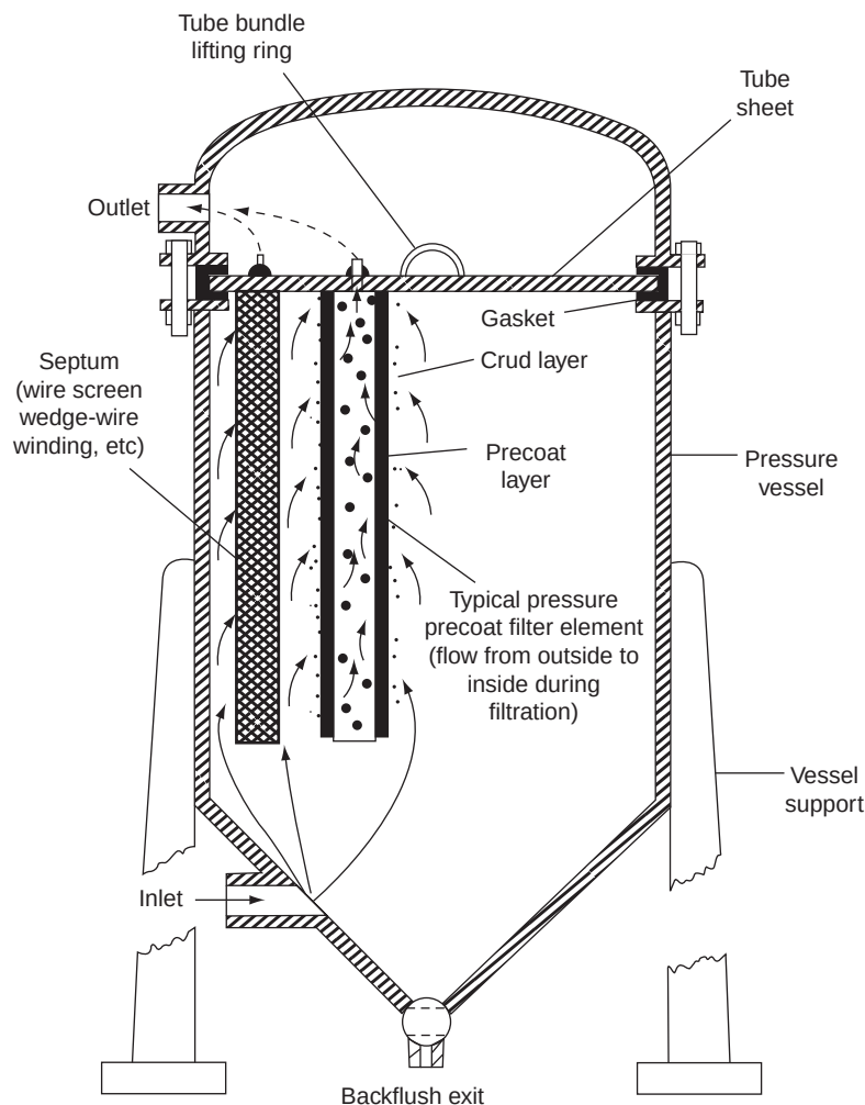
FIGURE 22.8 Disposal-cartridge filter unit used to purify water and collect LLW. (Courtesy ORNL.)
