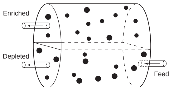
FIGURE 9.3 Gaseous diffusion stage.
