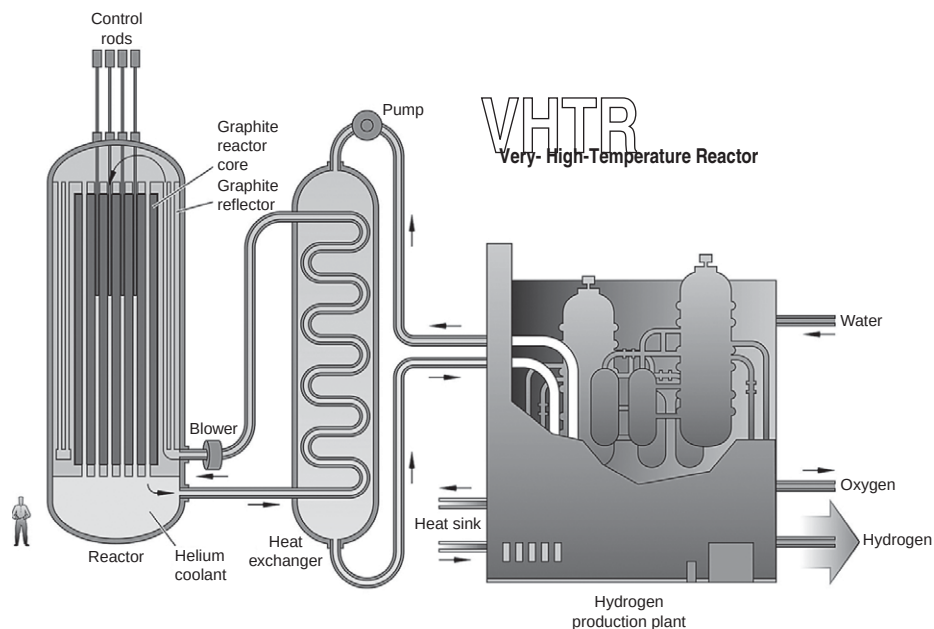
FIGURE 27.5 Very high temperature reactor with hydrogen processing unit. (Courtesy of DOE.)
