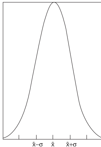
FIGURE 10.6 Gaussian distribution. The area between the limits x \pm \sigma is 68% of the total.
