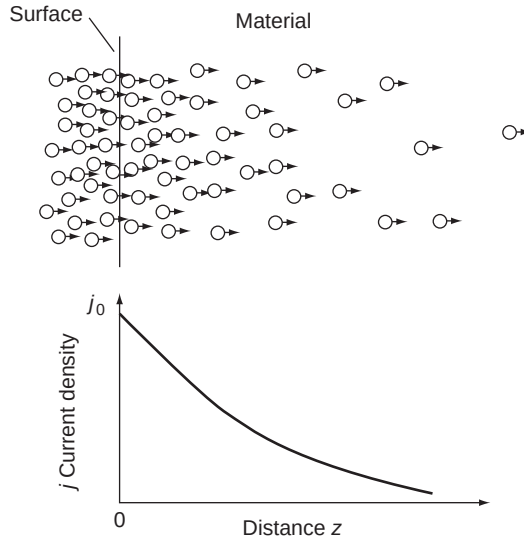
FIGURE 4.4 Neutron penetration and attenuation.
