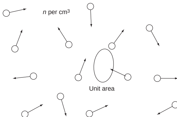
FIGURE 4.3 Particles in random motion.
