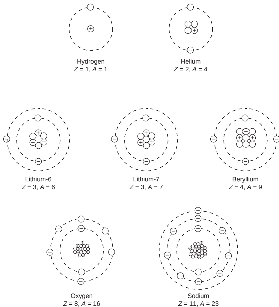
FIGURE 2.7 Atomic and nuclear structure.
