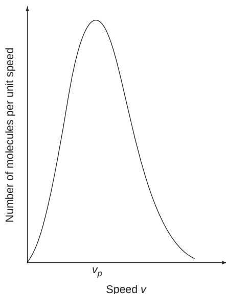
FIGURE 2.1 Distribution of molecular speeds.
