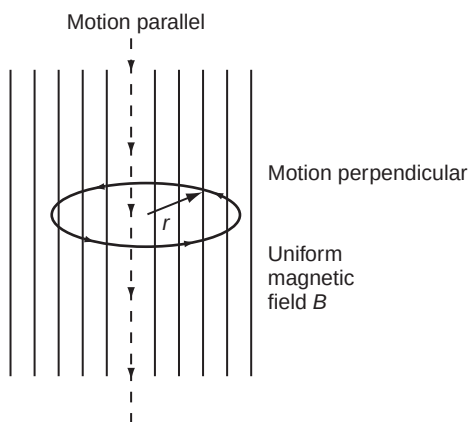
FIGURE 8.2 Electric charge motion in uniform magnetic field B .
