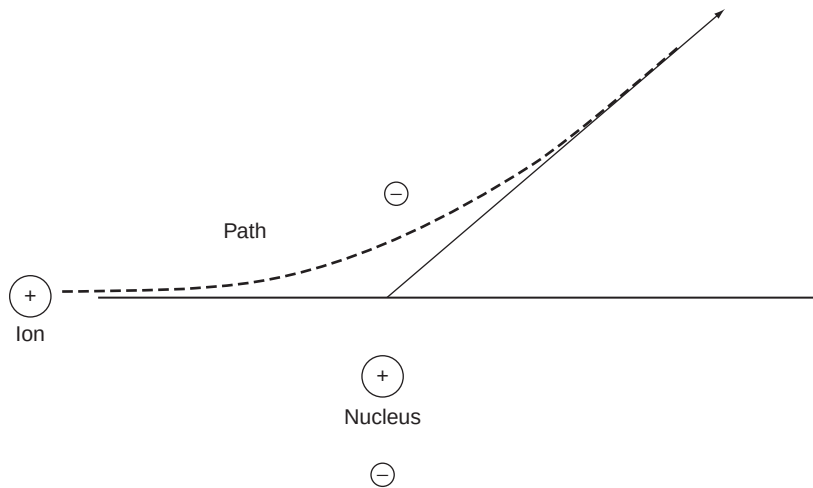
FIGURE 5.2 Interaction of heavy ion with nucleus.
