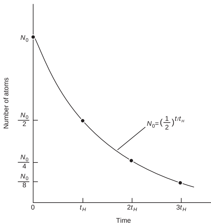
FIGURE 3.1 Radioactive decay.
