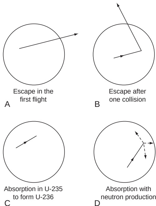
FIGURE 11.2 Neutron histories.
