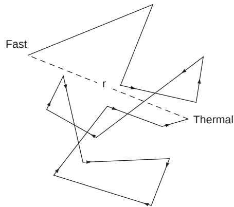
FIGURE 4.9 Neutron migration during slowing.
