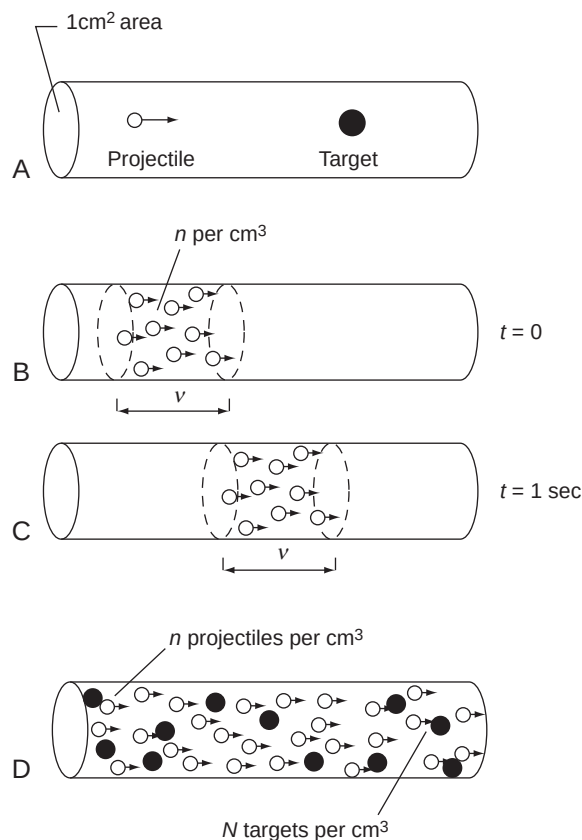
FIGURE 4.2 Particle collisions.
