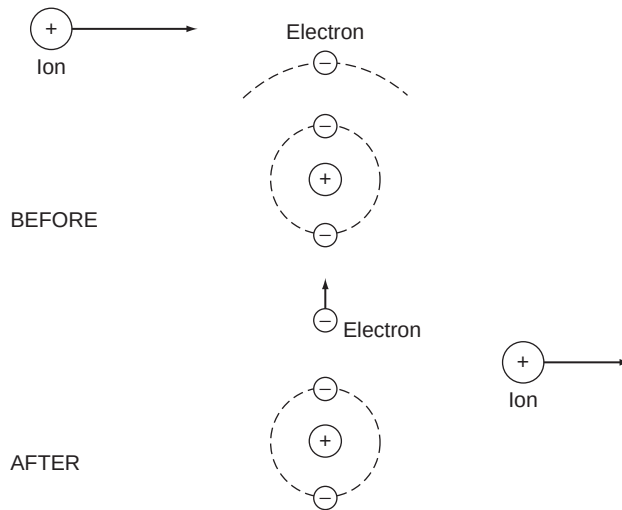
FIGURE 5.1 Interaction of heavy ion with electron.
