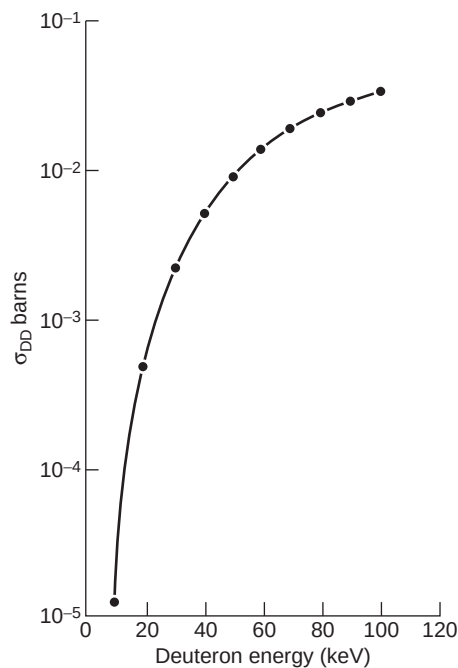
FIGURE 7.1 Cross section for D-D reaction.
