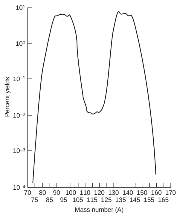
FIGURE 6.3 Yield of fission products according to mass number (Courtesy of T.R. England of Los Alamos National Laboratory).
