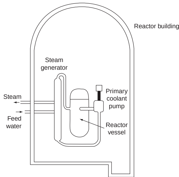
FIGURE 19.8 Reactor containment.
