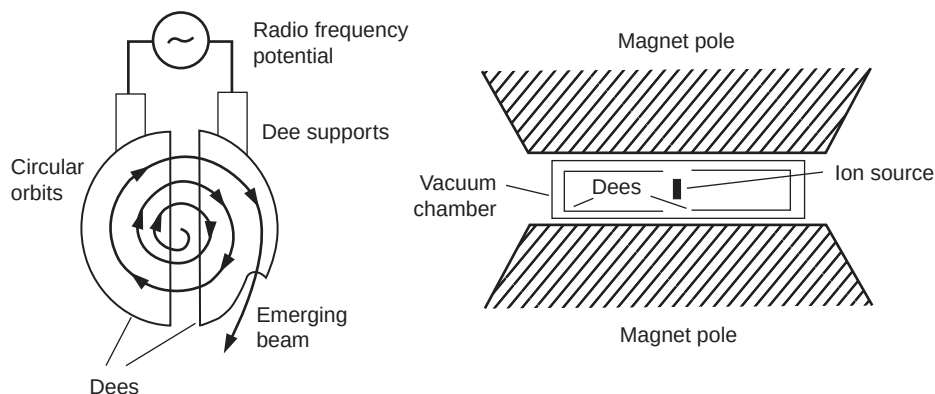
FIGURE 8.7 Cyclotron.
