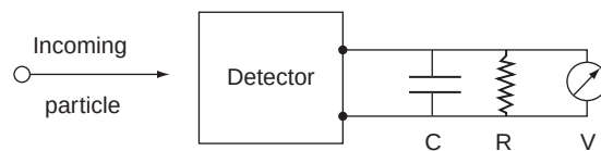
A Detector and electronic circuit
