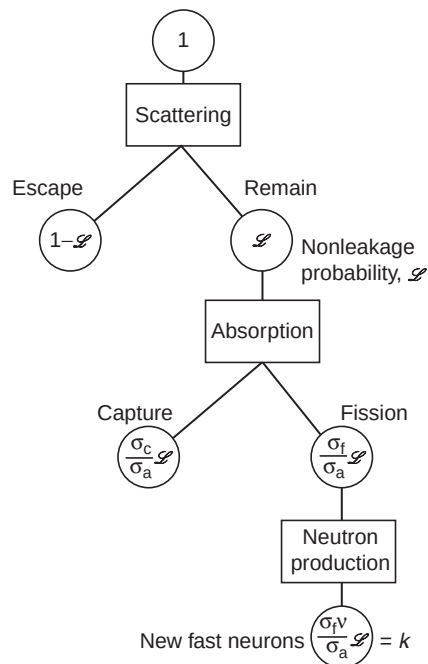
FIGURE 11.3 Neutron cycle in metal assembly.
