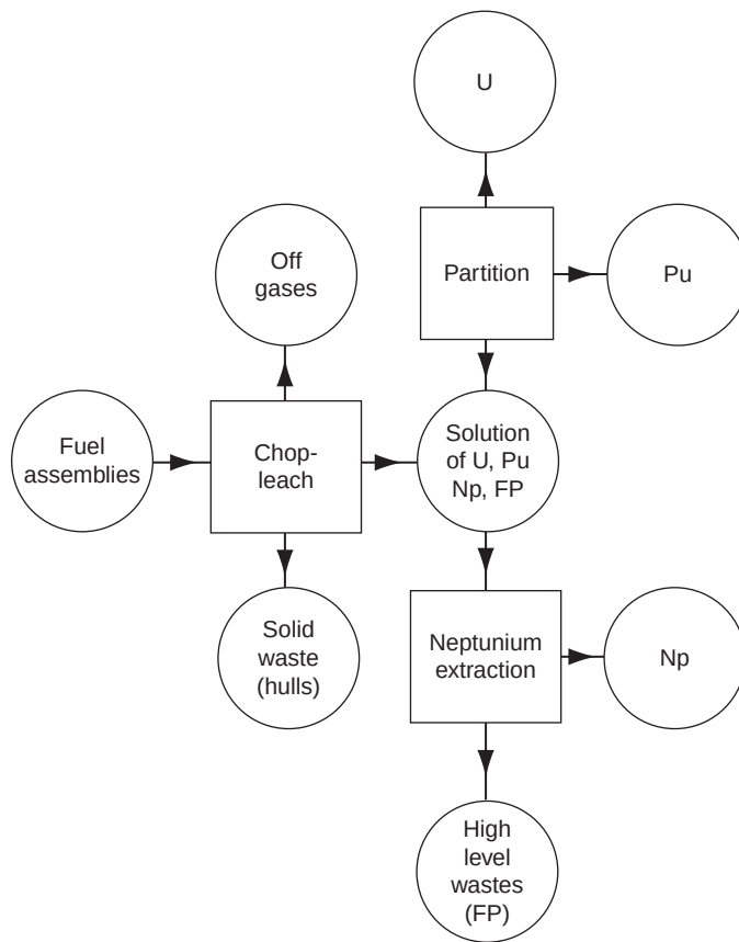
FIGURE 22.5 Simplified flowchart of nuclear fuel reprocessing.
