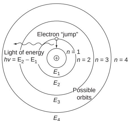
FIGURE 2.3 Electron orbits in hydrogen (Bohr theory).
