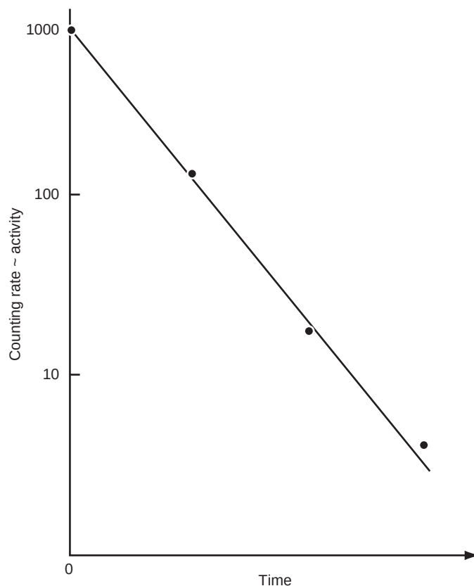
FIGURE 3.3 Activity plot.
