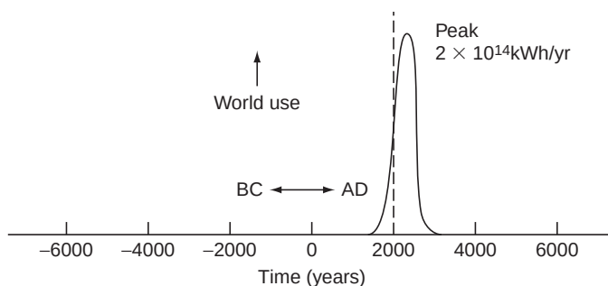
FIGURE 27.4 The epoch of fossil fuels. (Adapted from Energy Resources: A Report to The Committee on Natural Resources , M. King Hubbert, National Academy of Sciences – National Research Council, Washington, DC, 1962.)
