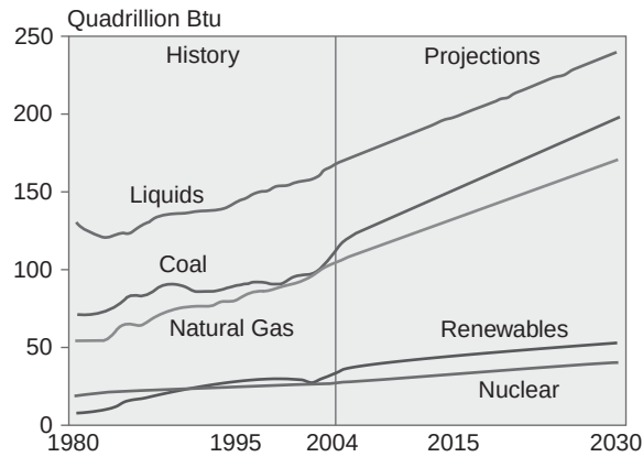
FIGURE 27.1 World energy consumption 1980–2030. Source: International Energy Outlook 2007.
