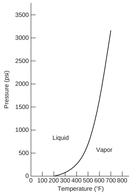
FIGURE 12.5 Relationship of pressure and temperature for water.
