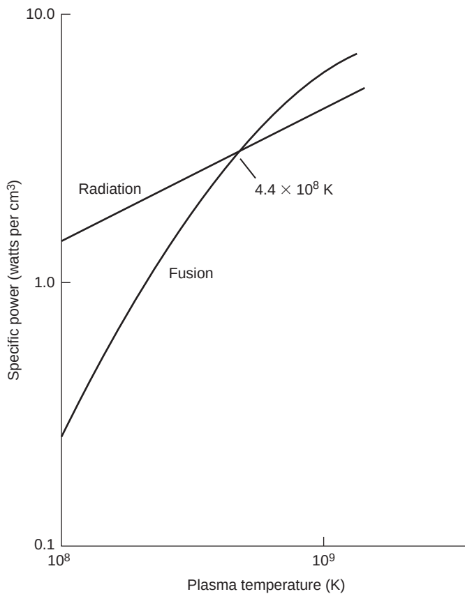
FIGURE 7.2 Fusion and radiation energies.
