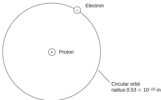
FIGURE 2.2 Hydrogen atom.
