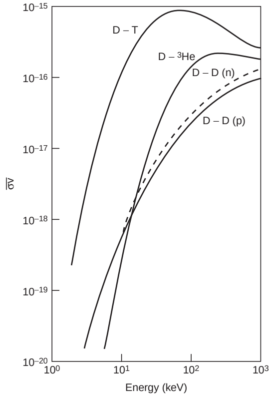
FIGURE 14.1 Reaction rates for fusion reactions. The quantity \bar{\sigma}v , the average over a Maxwellian distribution of cross section times speed, when multiplied by particle densities gives the fusion rate per unit volume.
