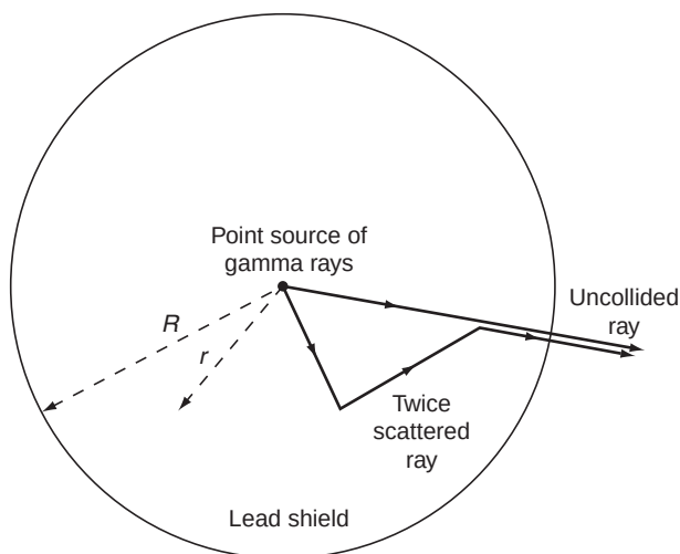
FIGURE 21.2 Buildup effect.
