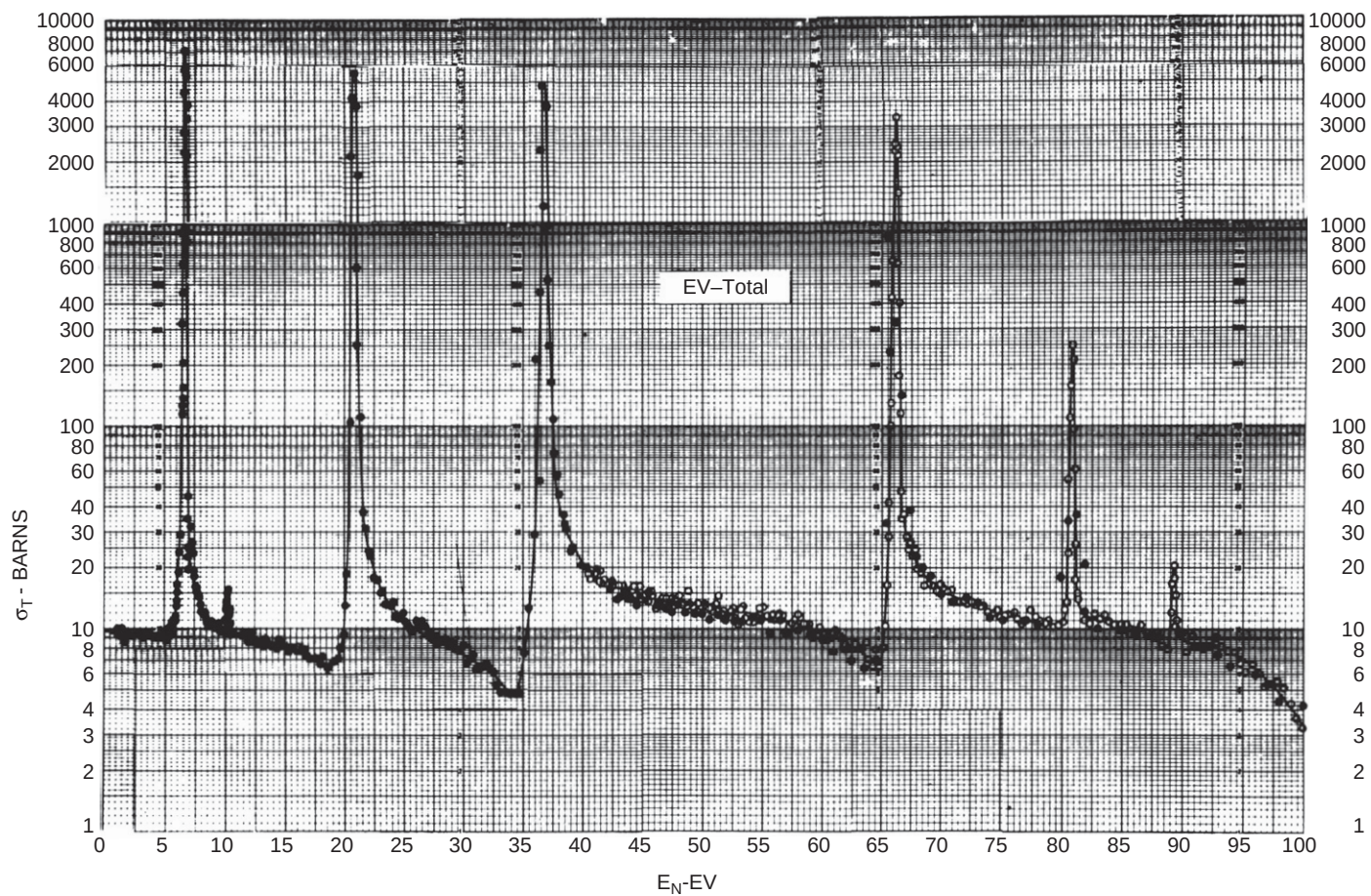
FIGURE 4.6 Cross section for natural uranium.
