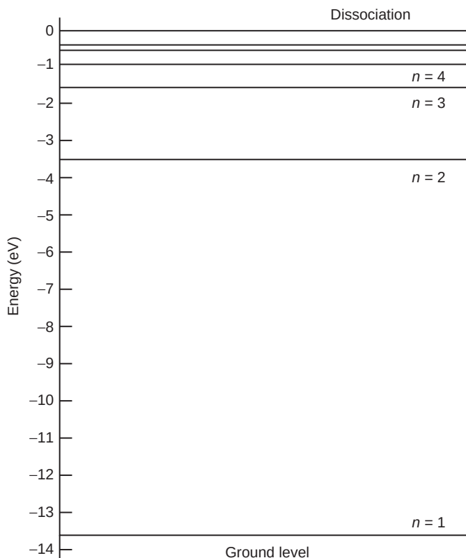
FIGURE 2.4 Energy levels in hydrogen atom.
