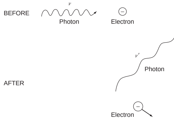
FIGURE 5.3 Photon electron scattering (Compton effect).
