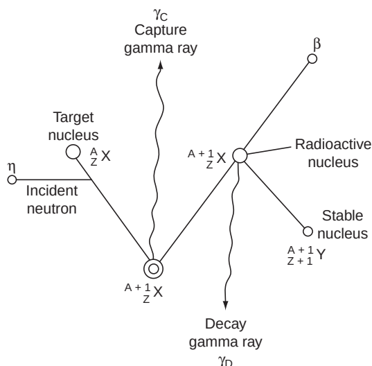
FIGURE 17.5 Nuclear reactions involved in neutron activation analysis (PGNAA) (Courtesy of Institute of Physics).
