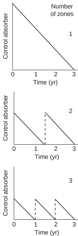
FIGURE 19.7 Reactor operation with different numbers of fuel zones. The initial control absorber varies inversely with the number of regions.
