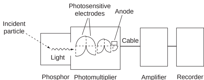
FIGURE 10.3 Scintillation detection system.
