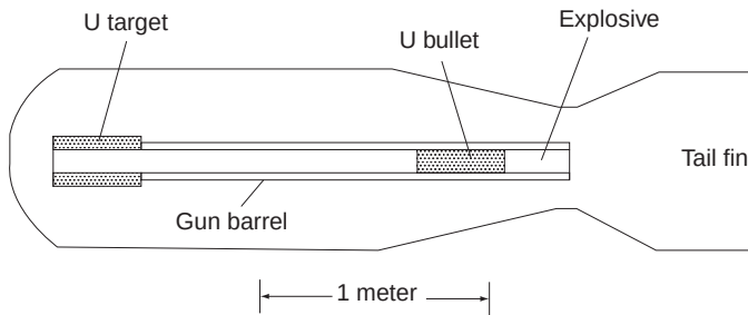
FIGURE 26.1 Uranium fission nuclear weapon, gun type Little Boy.
