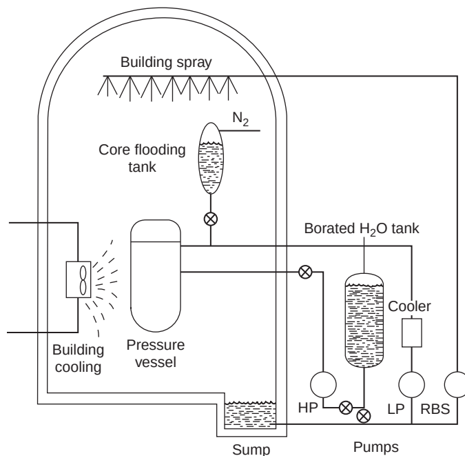
FIGURE 19.9 Emergency core cooling system. Pumps: HP, high pressure; LP, low pressure; RBS, reactor building spray.
