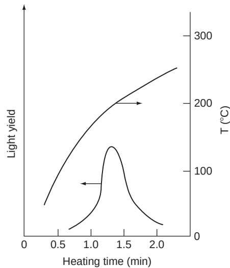
FIGURE 10.4 Glow curve of the phosphor \text{CaF}_2 .
