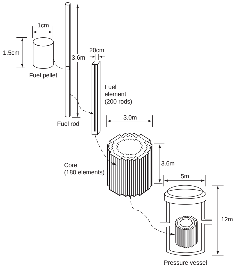
FIGURE 11.5 Reactor construction.
