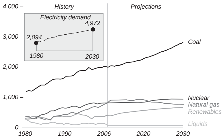
FIGURE 24.3 Energy generation by fuel, 1980–2030 (billion kWh). Source: Annual Energy Outlook 2008. DOE/EIA-0383(2008).
