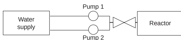
(A) Physical arrangement of pumping system
