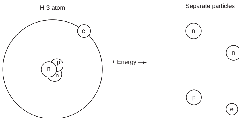
FIGURE 2.8 Dissociation of tritium.
