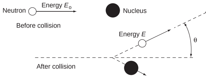
FIGURE 4.8 Neutron scattering and energy loss.
