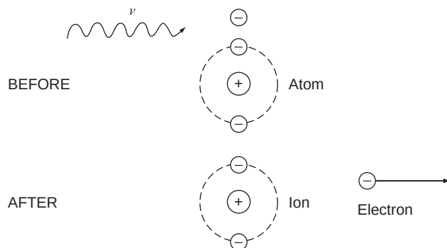
FIGURE 5.5 Photoelectric effect.
