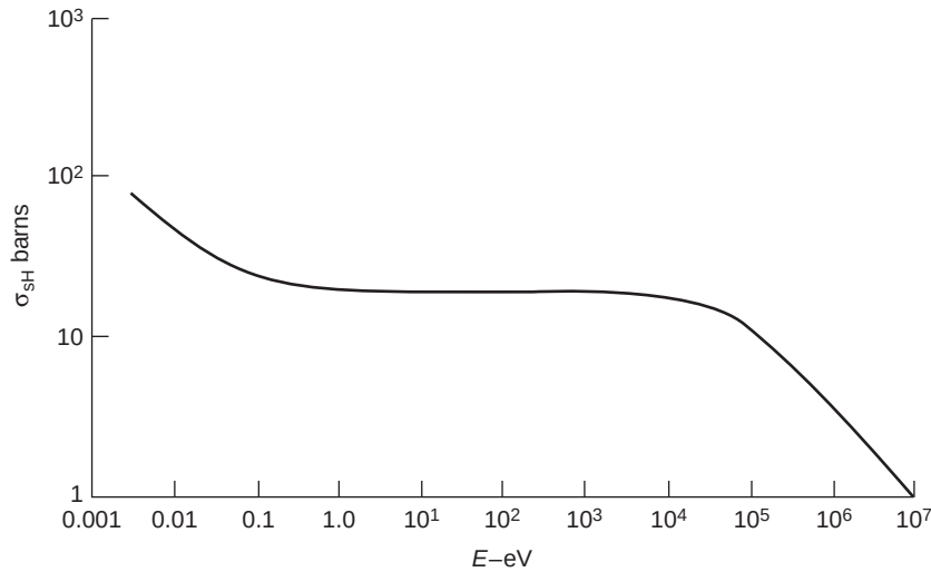
FIGURE 4.7 Scattering cross section for hydrogen.
