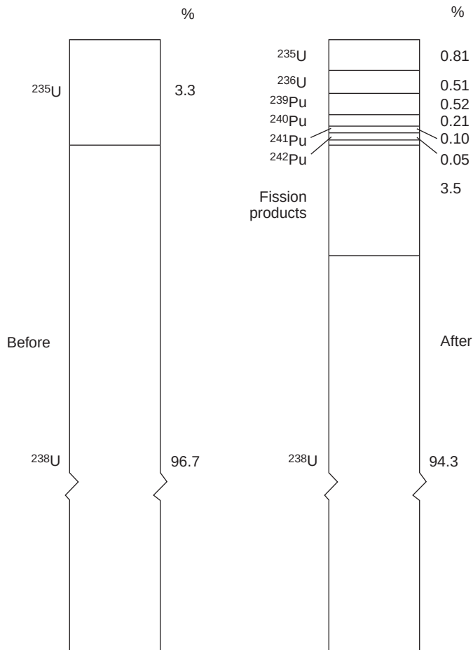
FIGURE 22.2 Composition of nuclear fuel before and after irradiation with neutrons in a reactor. (From Raymond L. Murray, Understanding Radioactive Waste , 2003, courtesy of Battelle Press, Columbus, OH.)
