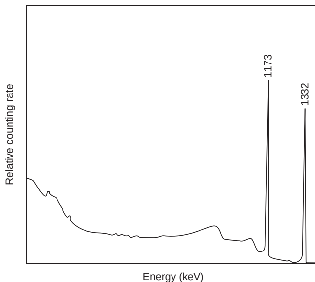
FIGURE 17.4 Analysis of gamma rays from cobalt-60. (Courtesy of Jack N. Weaver of North Carolina State University).
