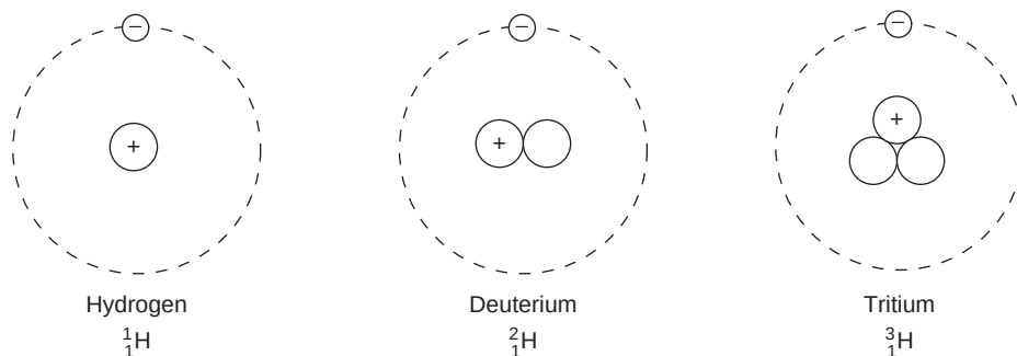
FIGURE 2.6 Isotopes of hydrogen.
