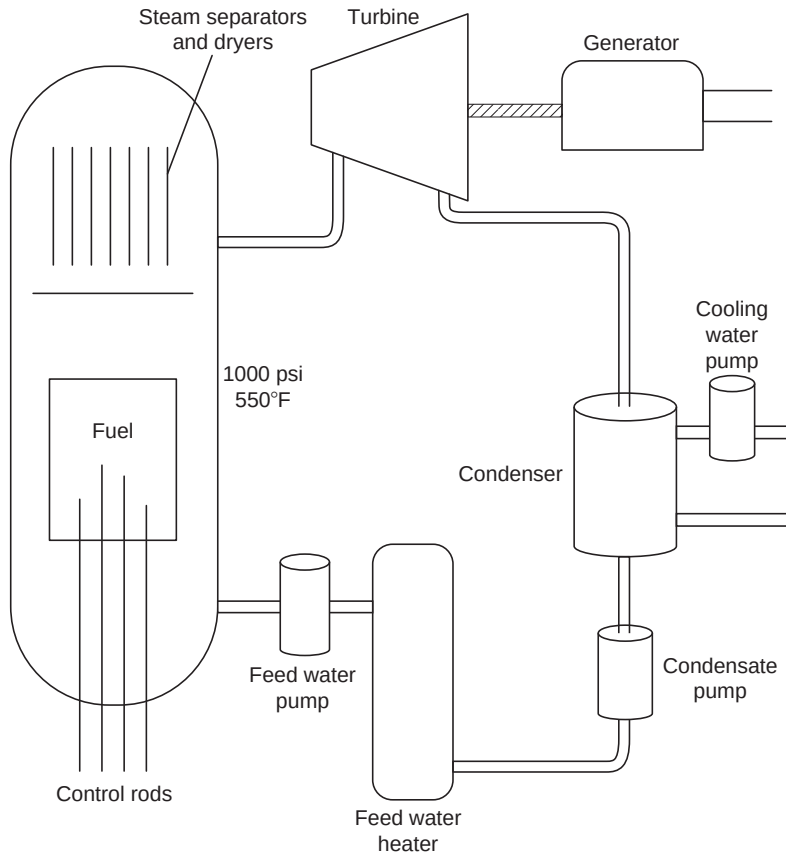
FIGURE 12.8 BWR system flow diagram.
