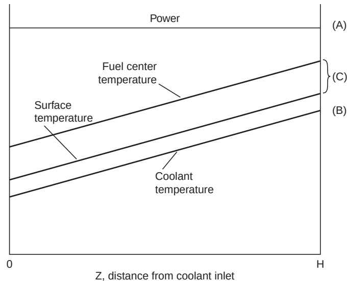
FIGURE 12.2 Temperature distributions along axis of reactor with uniform power.
