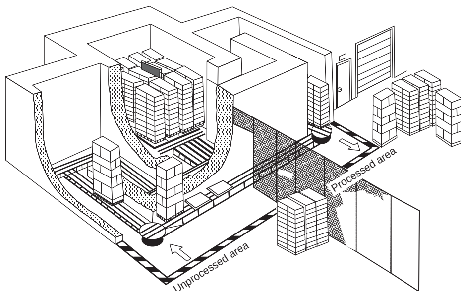
FIGURE 18.1 Gamma irradiation of Sterigenics International, at Haw River, NC. Pallets containing boxes of products move on a computer-controlled conveyor through a concrete maze past a gamma-emitting screen.
