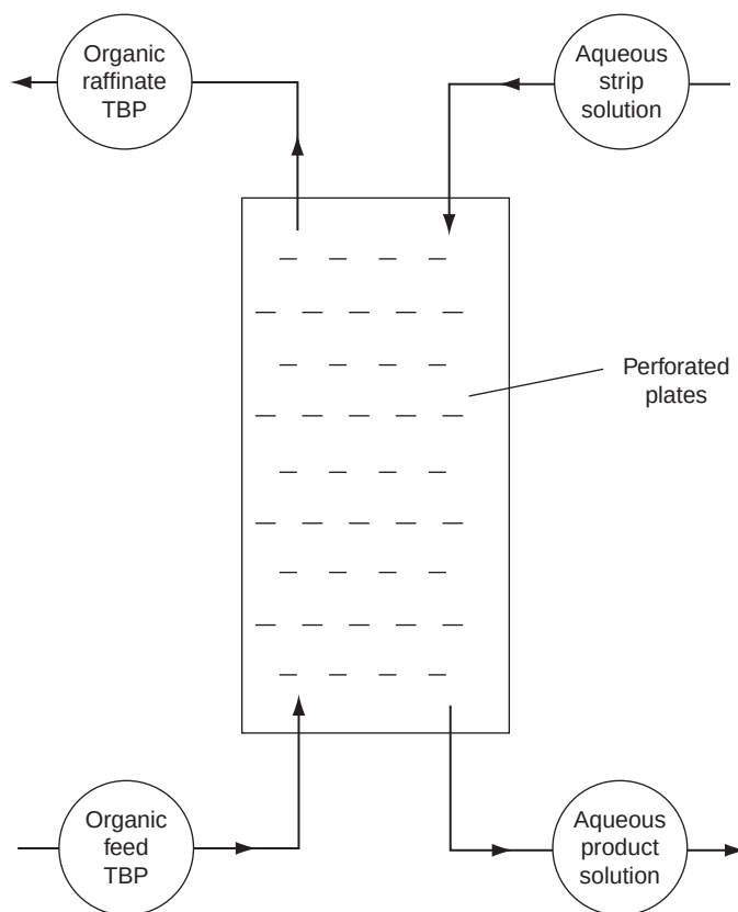
FIGURE 22.4 Solvent extraction by the Purex method.
