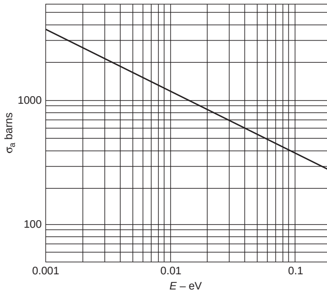
FIGURE 4.5 Absorption cross section for elemental boron.
