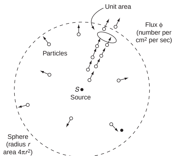
FIGURE 21.1 Inverse square spreading of radiation.
