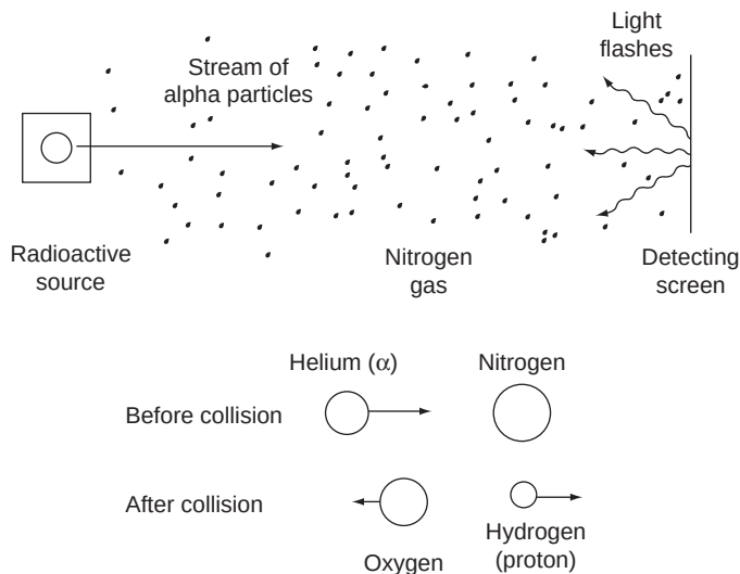
Rutherford's experiment
