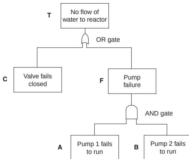
(B) Fault tree
