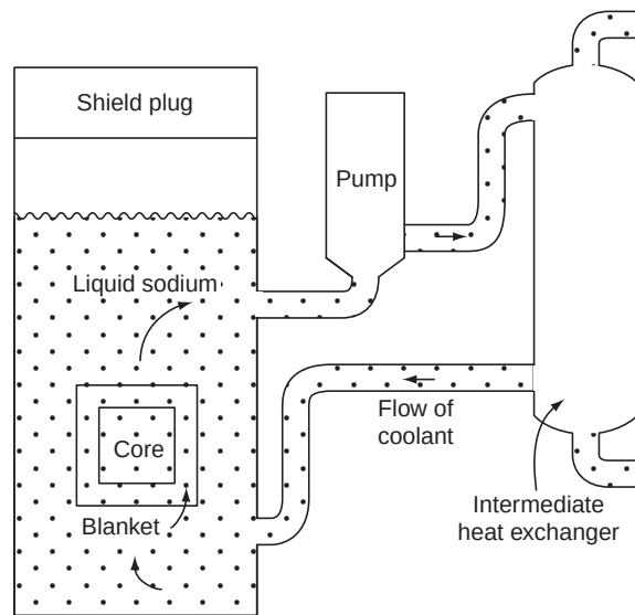
FIGURE 13.1 Loop system for LMFBR.
