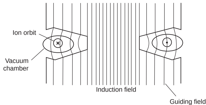
FIGURE 8.8 Betatron.
