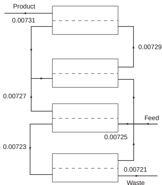
FIGURE 9.4 Gaseous diffusion cascade.
