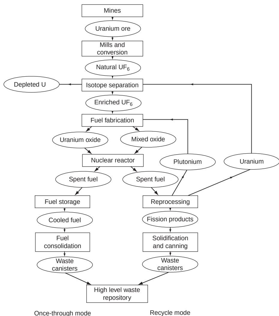
FIGURE 22.1 Nuclear fuel cycles. The once-through shown on the left is used in the United States; the recycle shown on the right is used in other countries.
