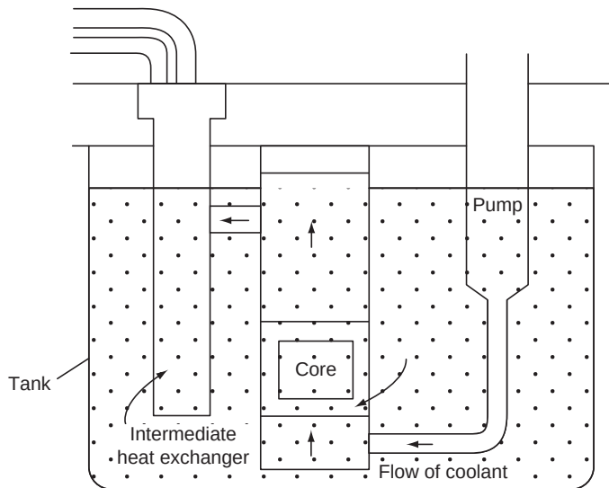
FIGURE 13.2 Pot system for LMFBR.
