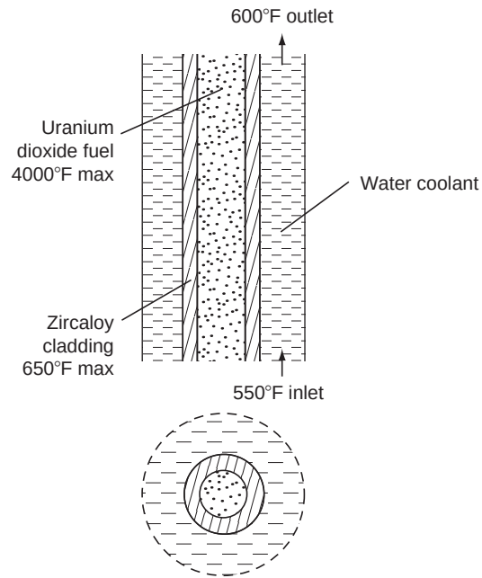
FIGURE 12.4 Reactor channel heat removal.
