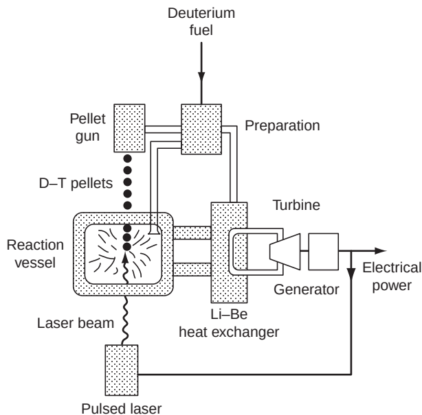
FIGURE 14.6 Laser-fusion reactor.
