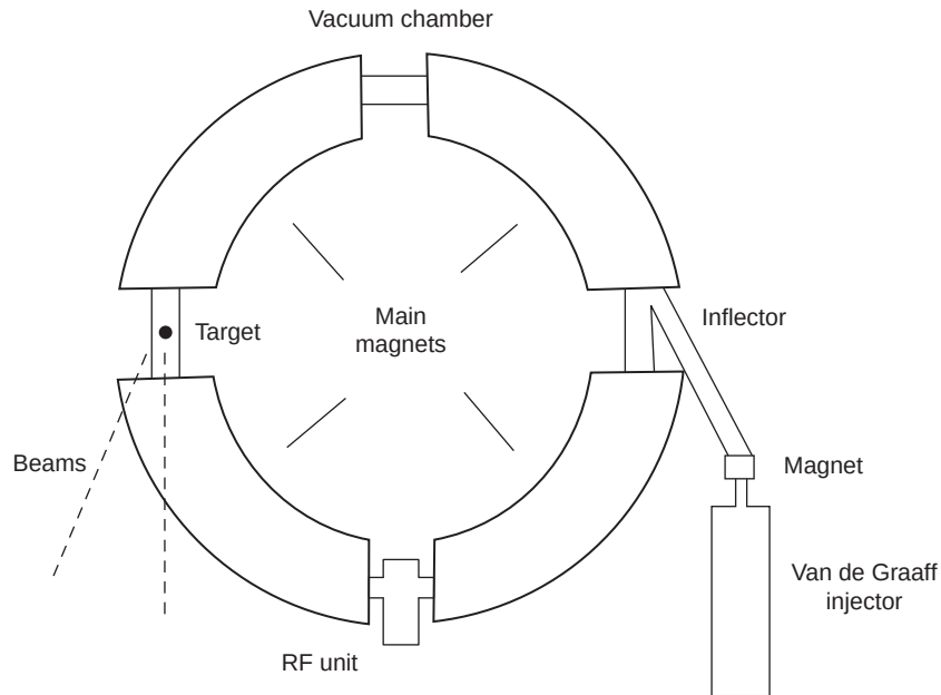
FIGURE 8.9 Cosmotron. Synchrotron at Brookhaven National Laboratory.
