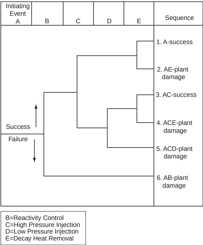
FIGURE 19.10 Simple event tree (After NUREG/CR-4350, Vol.1).
