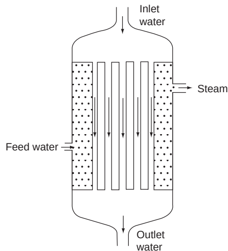
FIGURE 12.6 Heat exchanger or steam generator.
