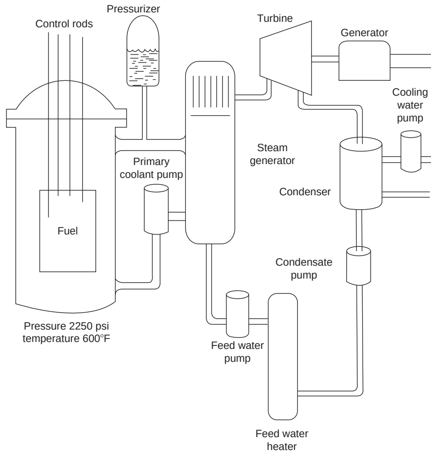
FIGURE 12.7 PWR system flow diagram.
