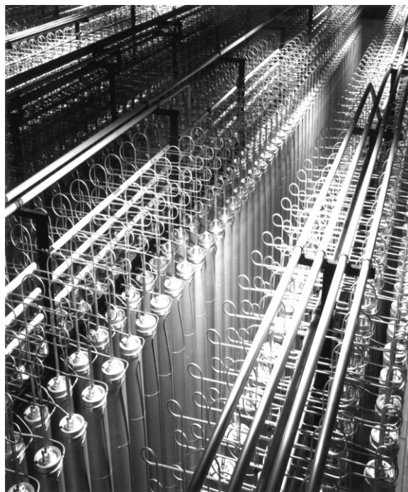
FIGURE 9.7 One of the centrifuge enrichment halls of the plant at Almelo, The Netherlands. (Courtesy Urenco, Ltd.).
