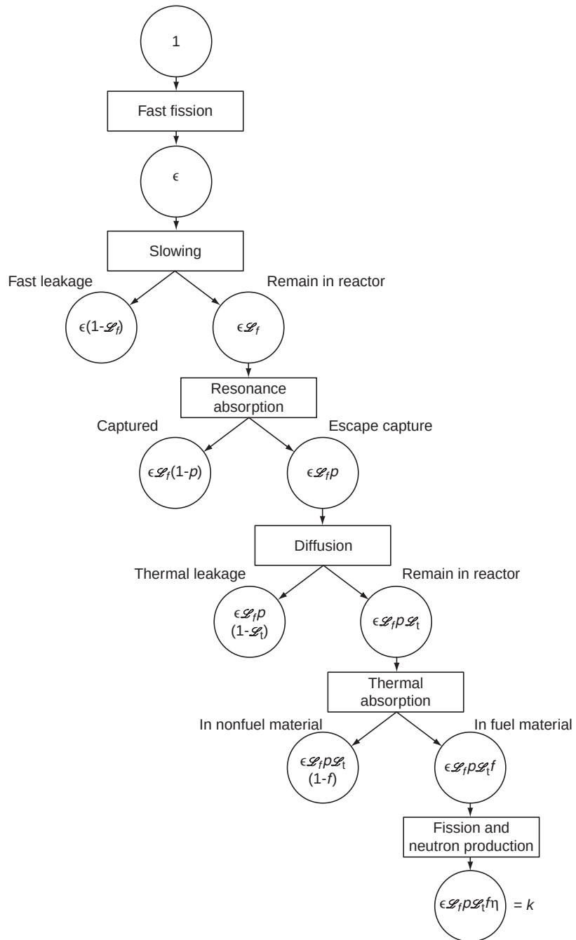
FIGURE 11.4 Neutron cycle in thermal reactor.
