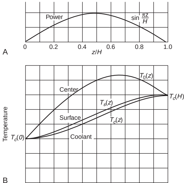
FIGURE 12.3 Temperature distributions along channel with sine function power.
