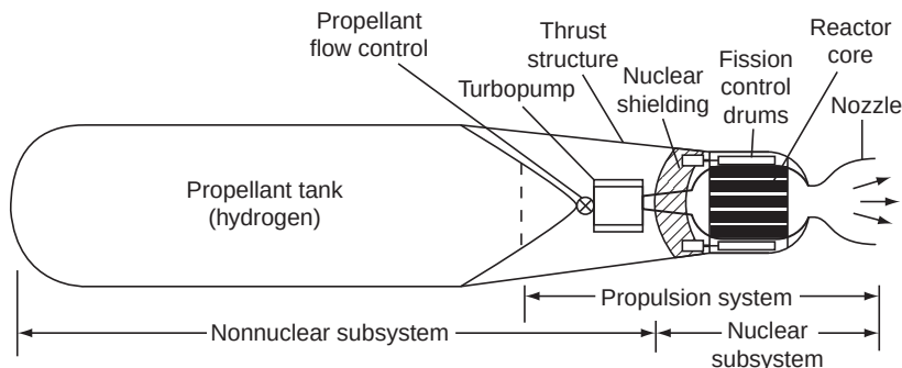
FIGURE 20.2 Nuclear-thermal rocket system. Hydrogen stored in liquid form is heated in the solid core and expelled as propellant. (Courtesy Gary Bennett).
