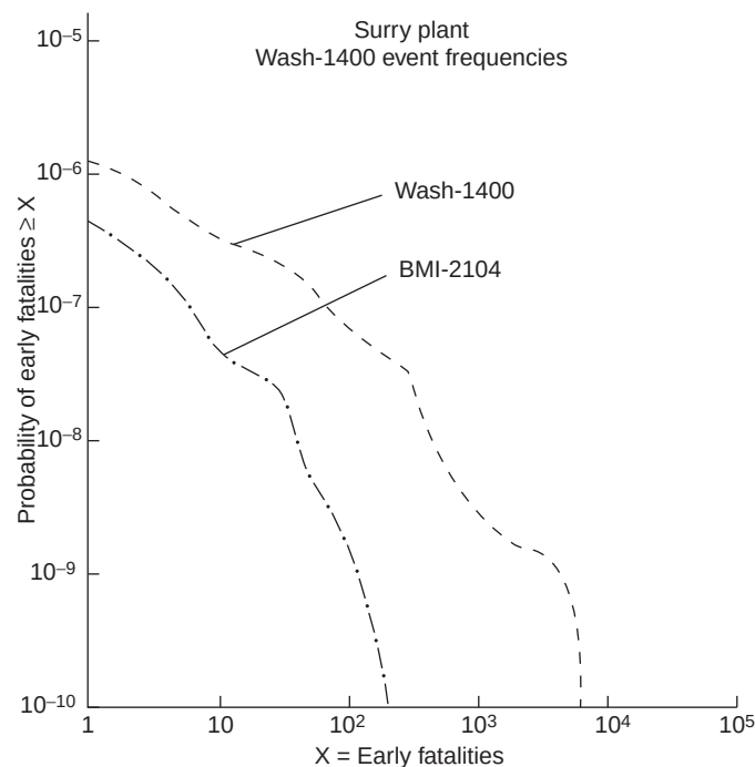
FIGURE 19.12 Distribution function for the Surry, Virginia, plant. The probabilities for various numbers of early fatalities are shown (Adapted from NUREG-0956).
