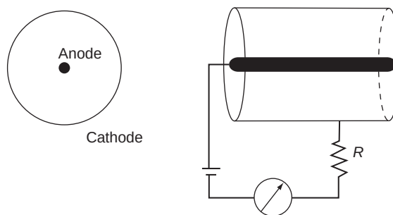
FIGURE 10.1 Basic detector.
