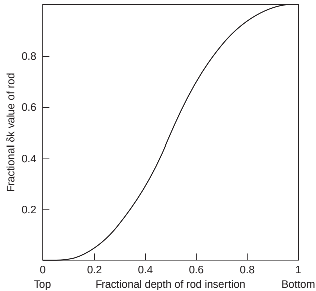
FIGURE 19.5 Control rod worth as it depends on depth of insertion in an unreflected reactor core.
