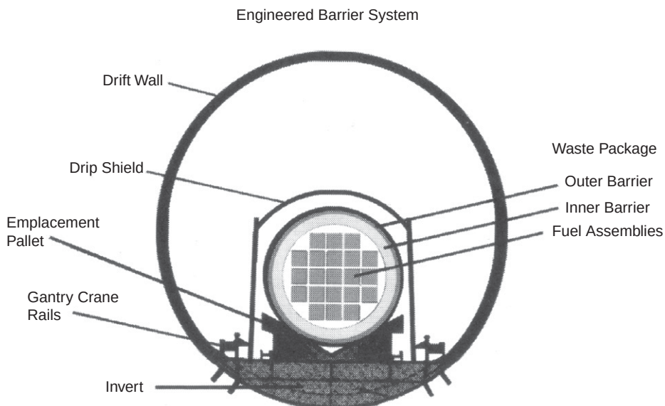
FIGURE 22.7 Spent fuel at Yucca Mountain.
