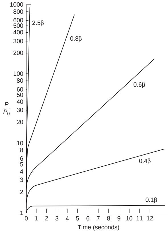
FIGURE 19.2 Effect of delayed neutrons.
