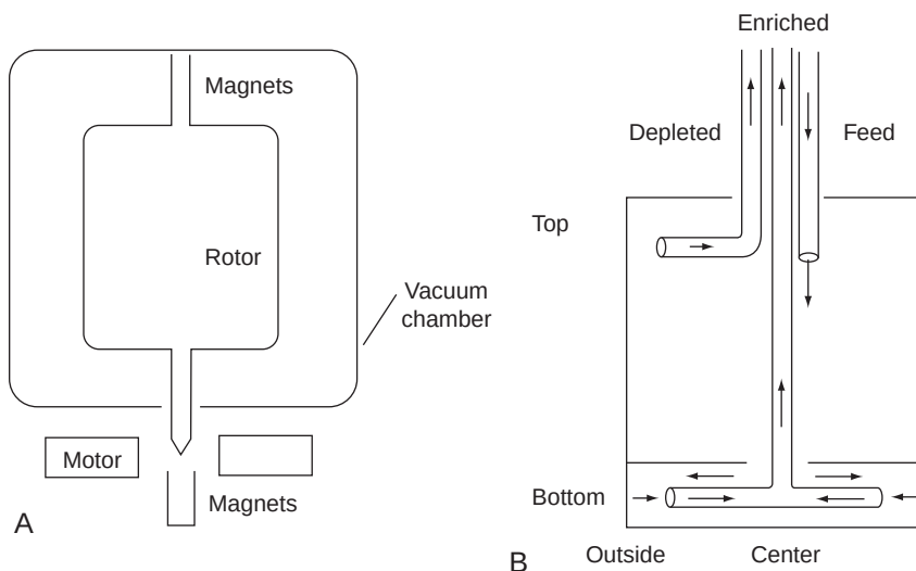
FIGURE 9.6 (A) Gas centrifuge. (B) Gas streams in centrifuge.
