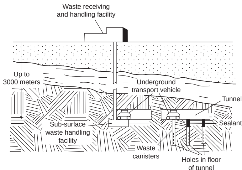
FIGURE 22.6 Nuclear waste isolation by geologic emplacement.
