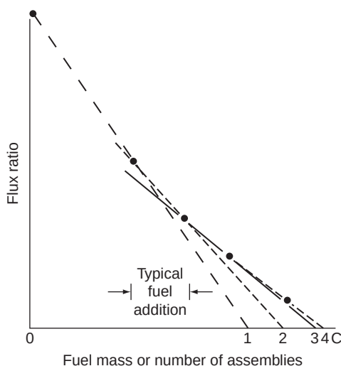
FIGURE 19.1 Critical experiment.
