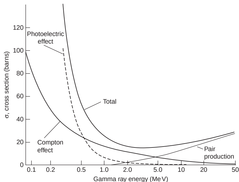
FIGURE 5.4 Gamma ray cross sections in lead, Pb. Plotted from data in National Bureau of Standards report NSRDS-NSB-29.
