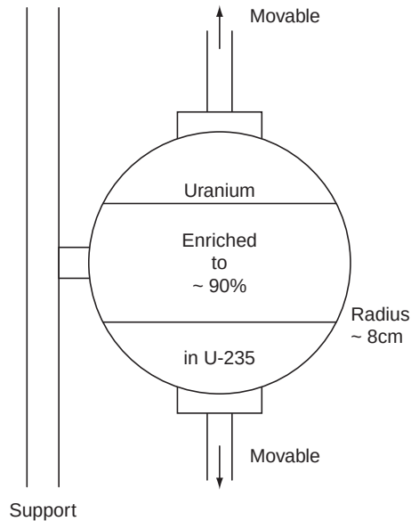
FIGURE 11.1 Fast metal assembly “Lady Godiva.”
