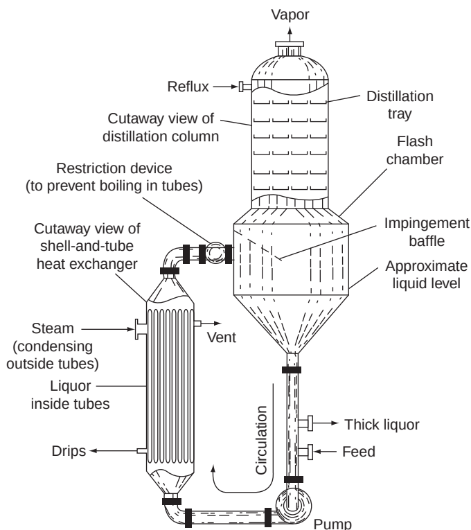
FIGURE 22.9 Natural-circulation evaporator used to concentrate LLW. (Courtesy ORNL.)
