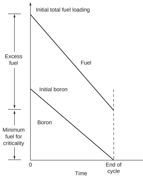
FIGURE 11.6 Reactor control during fuel consumption in power reactor.
