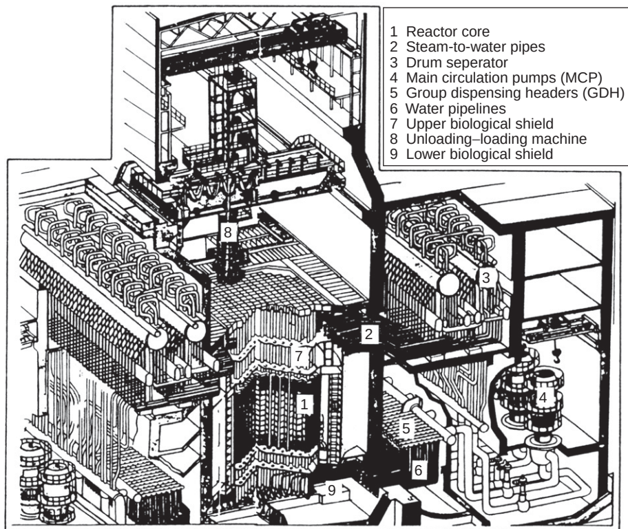
FIGURE 19.13 The Chernobyl reactor and building before the 1986 accident.
