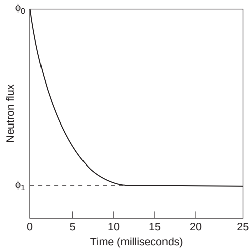
FIGURE 19.6 Neutron flux variation with time in the rod-drop method of measuring reactivity.
