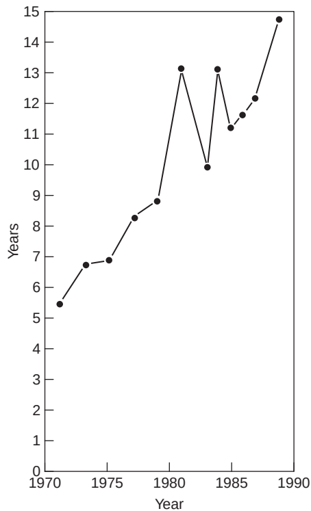
FIGURE 24.2 Construction times for nuclear power plants. Adapted from DOE/EIA-0439(84).
