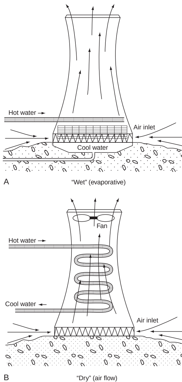
FIGURE 12.10 Cooling tower (From "Thermal Pollution and Aquatic Life" by John R. Clark, Scientific American , March 1969).
