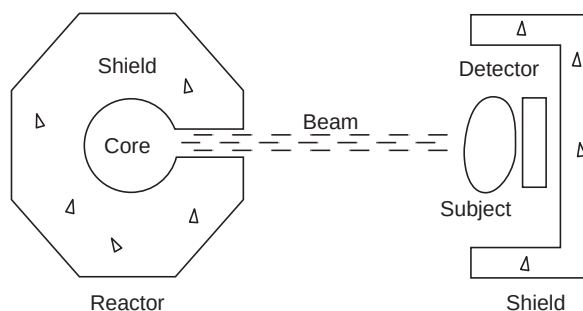
FIGURE 17.6 Schematic diagram of a thermal neutron radiography unit. Source can be an accelerator, a reactor, or a radioisotope.
