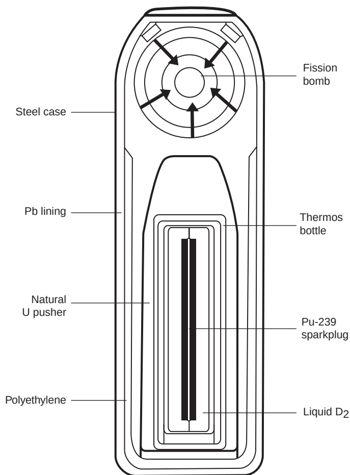
FIGURE 26.3 Thermonuclear weapon. (Adapted from Rhodes, see References .)
