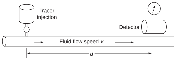
FIGURE 17.1 Tracer measurement of flow rate.
