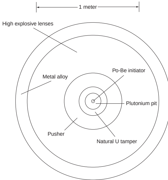
FIGURE 26.2 Plutonium fission nuclear weapon, implosion type Fat Man.
