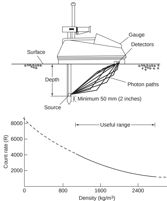
FIGURE 17.7 Direct-transmission radiation gauge to measure soil density. (Courtesy of Troxler Electronic Laboratories, Inc).
