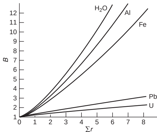
FIGURE 21.3 Buildup factors, 1 MeV gammas. B for concrete and aluminum are about the same.
