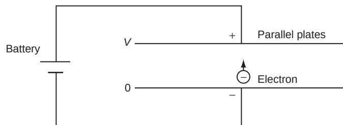
FIGURE 8.1 Capacitor as accelerator.
