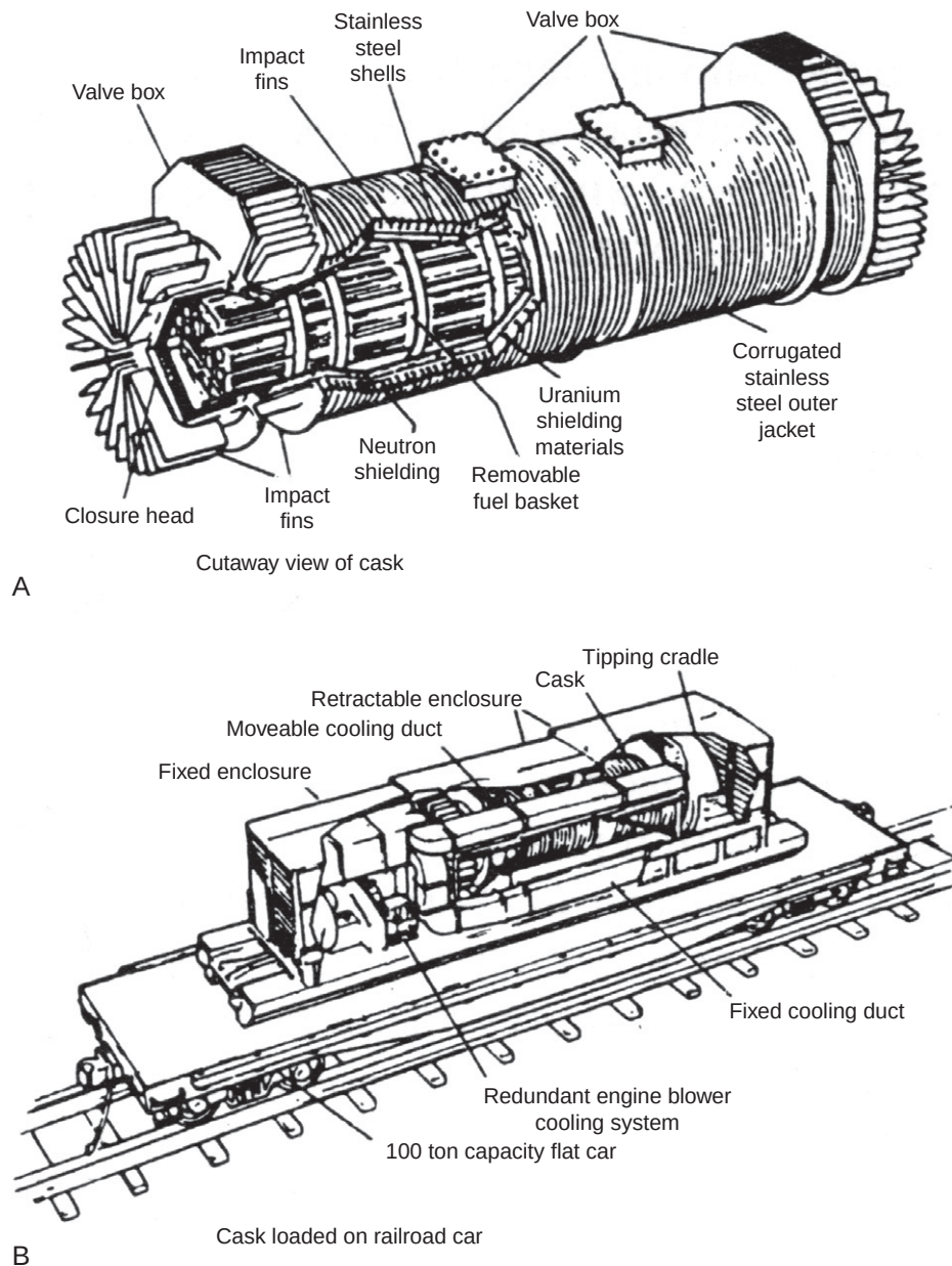
FIGURE 22.3 Spent fuel shipping cask. (Courtesy of General Electric Company.)
