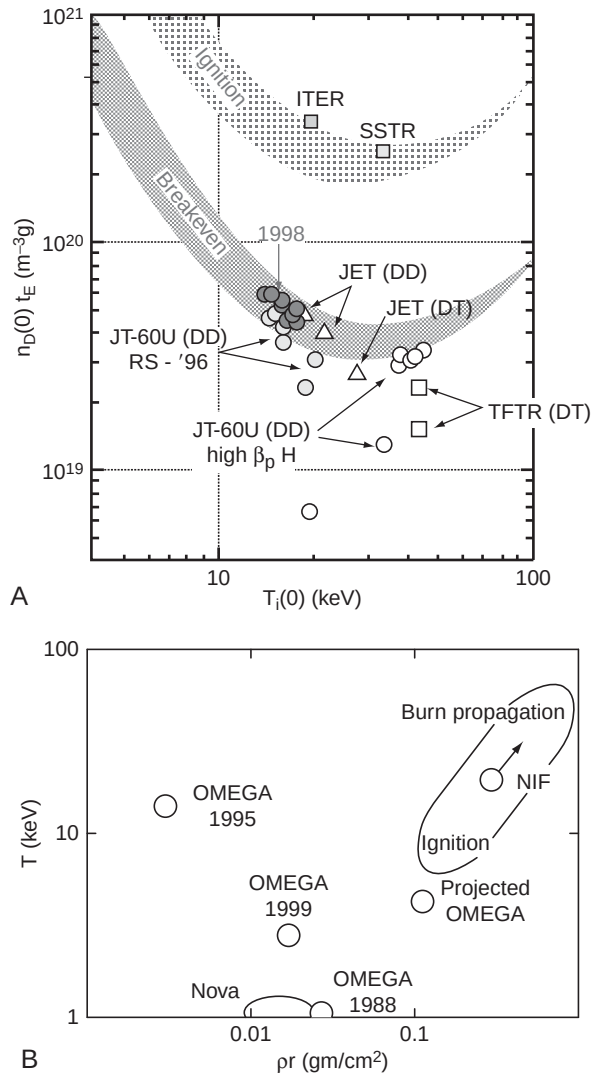
FIGURE 14.7 (A) Progress towards a practical MCF reactor. (Courtesy Japan Atomic Energy Research Institute. Thanks are due Robert Heeter). (B) Progress towards a practical ICF reactor. (Courtesy Lawrence Livermore National Laboratory. Thanks are due to John Soures and Alan Wootton.)
