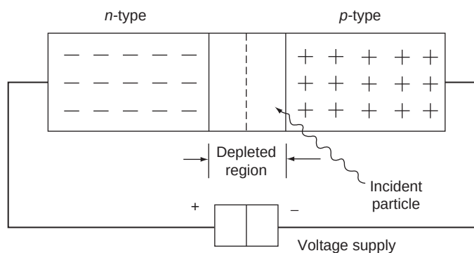
FIGURE 10.5 Solid-state n-p junction detector.
