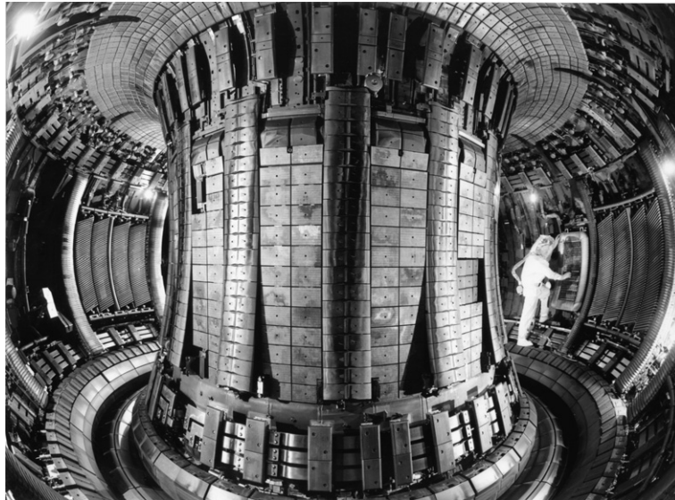
FIGURE 14.4 Interior of tokamak fusion reactor Joint European Torus at Culham, U.K. (Courtesy Joint European Torus).
