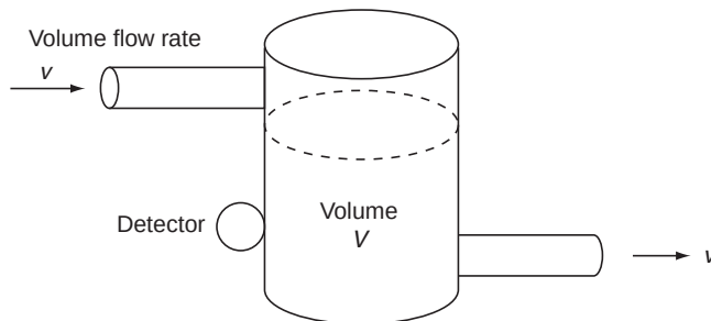
FIGURE 17.2 Flow decay.
