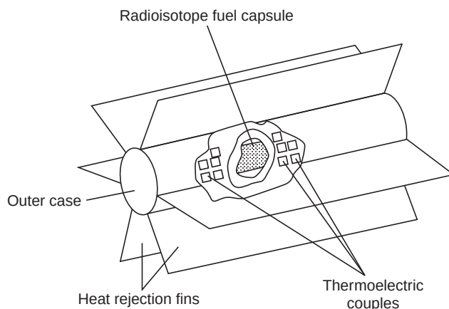
FIGURE 20.3 Isotopic electrical power generator. (SNAP-27 used in Apollo-12 mission).
