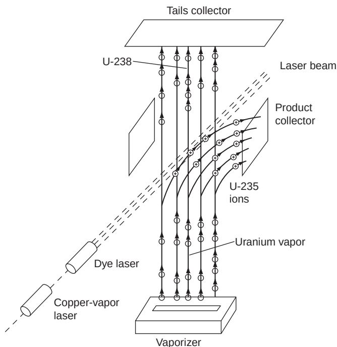
FIGURE 9.8 Atomic vapor laser isotopic separation.
